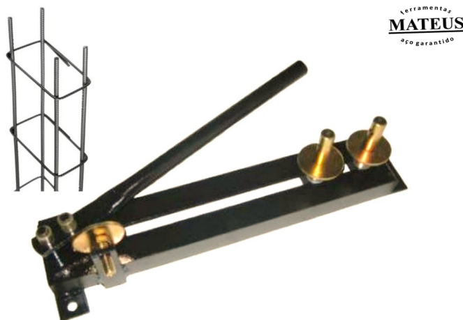
Ref. 002.1699 MAQUINA V/ ESTRIBOS 10 \ 12 m/m
