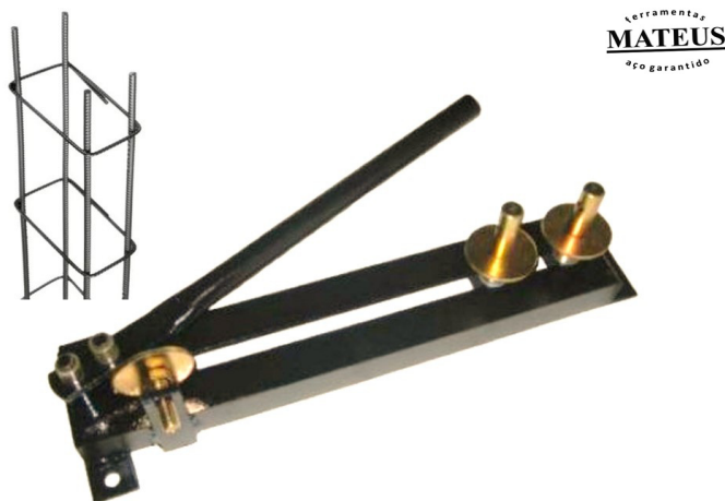
Ref. 002.1700 MAQUINA V/ ESTRIBOS 6 \ 8 m/m
